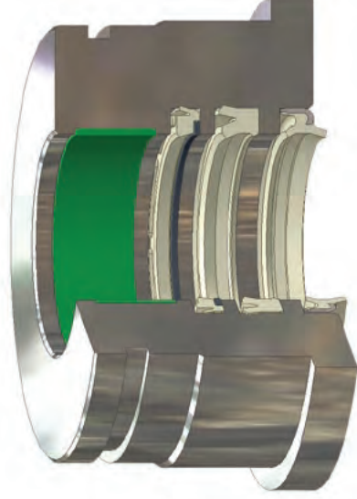
BT Installed in Rod Gland
