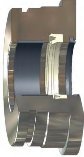
B3 Installed in Rod Gland
