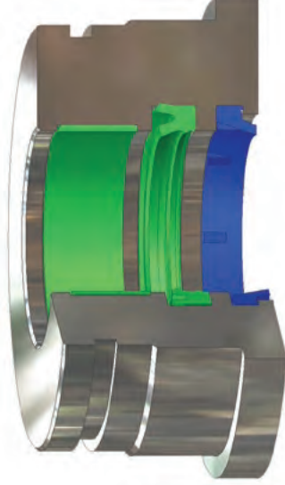
BS Installed in Rod Gland
