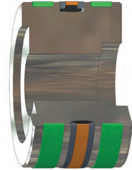
CT installed in Piston Gland
