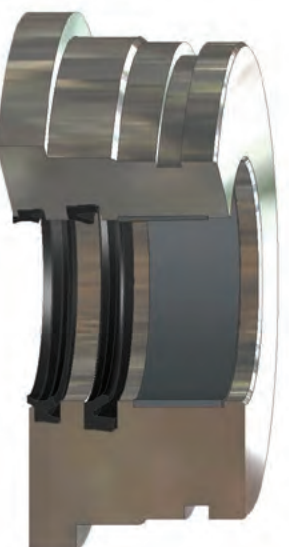
Rod sealing system comprised of PDW machined wear ring, E5 u-cup and 8600 wiper
