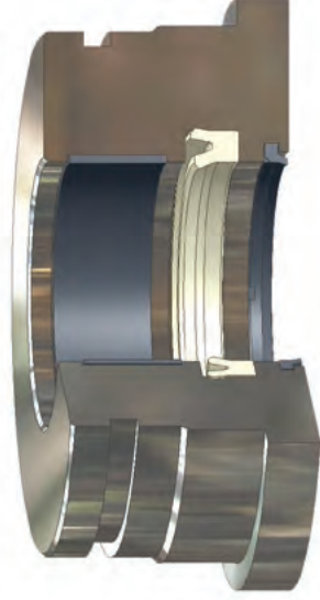
SH959 installed in Rod Gland
