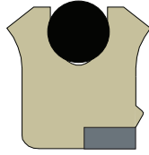
BD Cross-Section with Back-up
