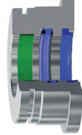
BD Installed in Rod Gland
