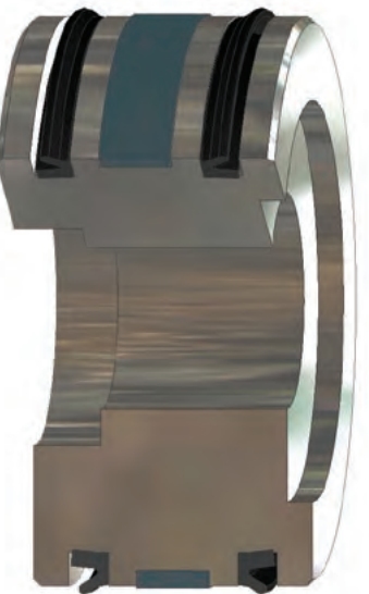
Piston sealing system comprised of PDW machined wear rings and E4 piston u-cups
