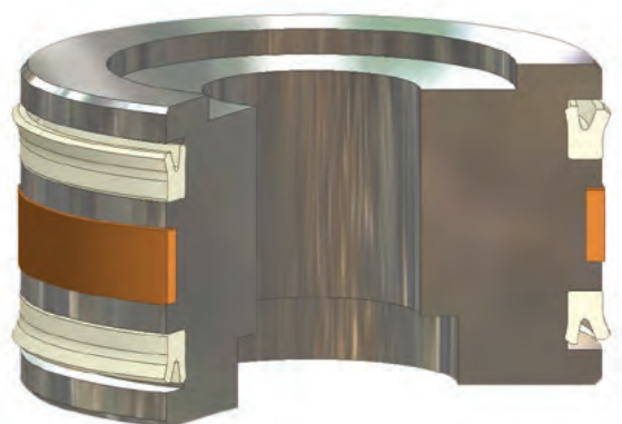
Piston sealing system comprised of PDT wear strip and B7 piston u-cups
