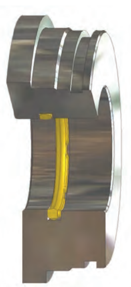
V6 Installed in Rod Gland
