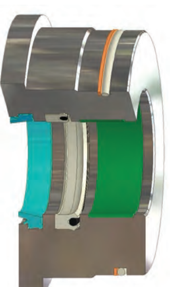
5100 installed in Rod Gland
